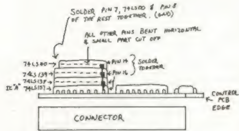
Illustration E: IC Stack
